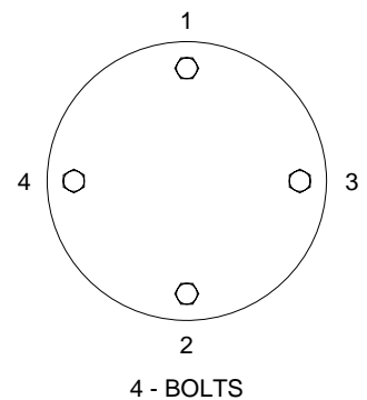
Figure 'B' EXAMPLE OF BOLT TORQUE SEQUENCE
